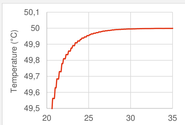
Figure 4. Temperature never overpasses setpoint
