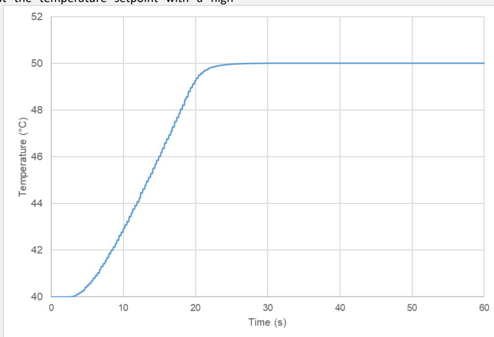
Figure 3. Regulation curve of a high stable blackbody
