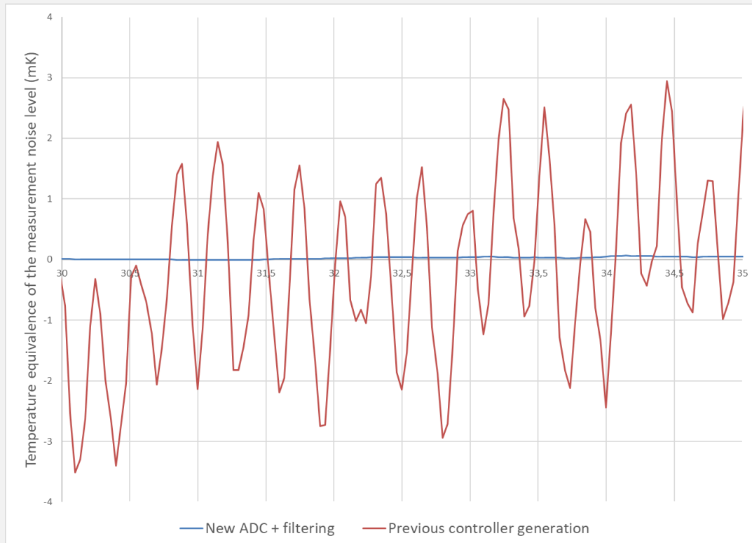
Figure 1. Noise level in mK before and after noise reduction
