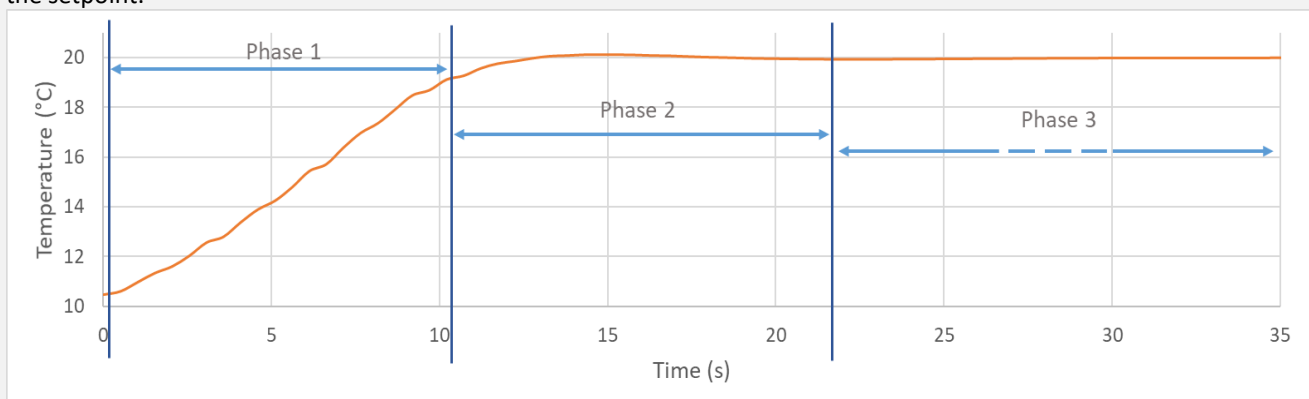
Figure 2. The three phases of the temperature regulation
