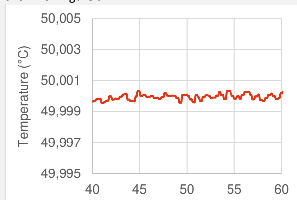
Figure 5. Long term regulation phase
